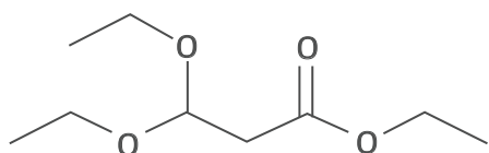
Ethyl 3,3-diethoxypropionate Cas No: 10601-80-6
